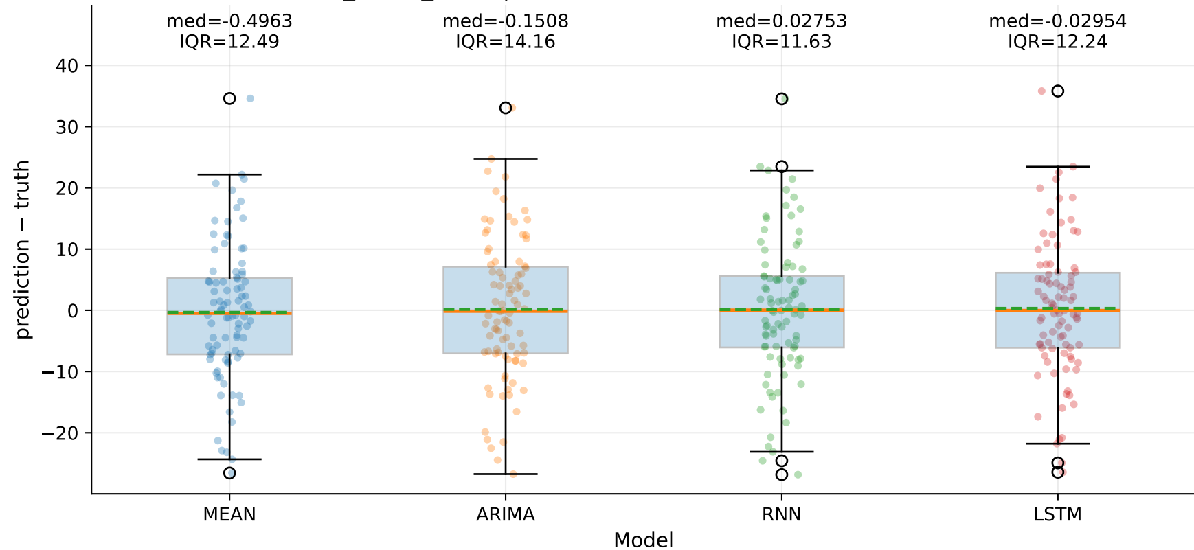
M7_YHUR_SLUR | Signed error by model — TSE (step=1)
