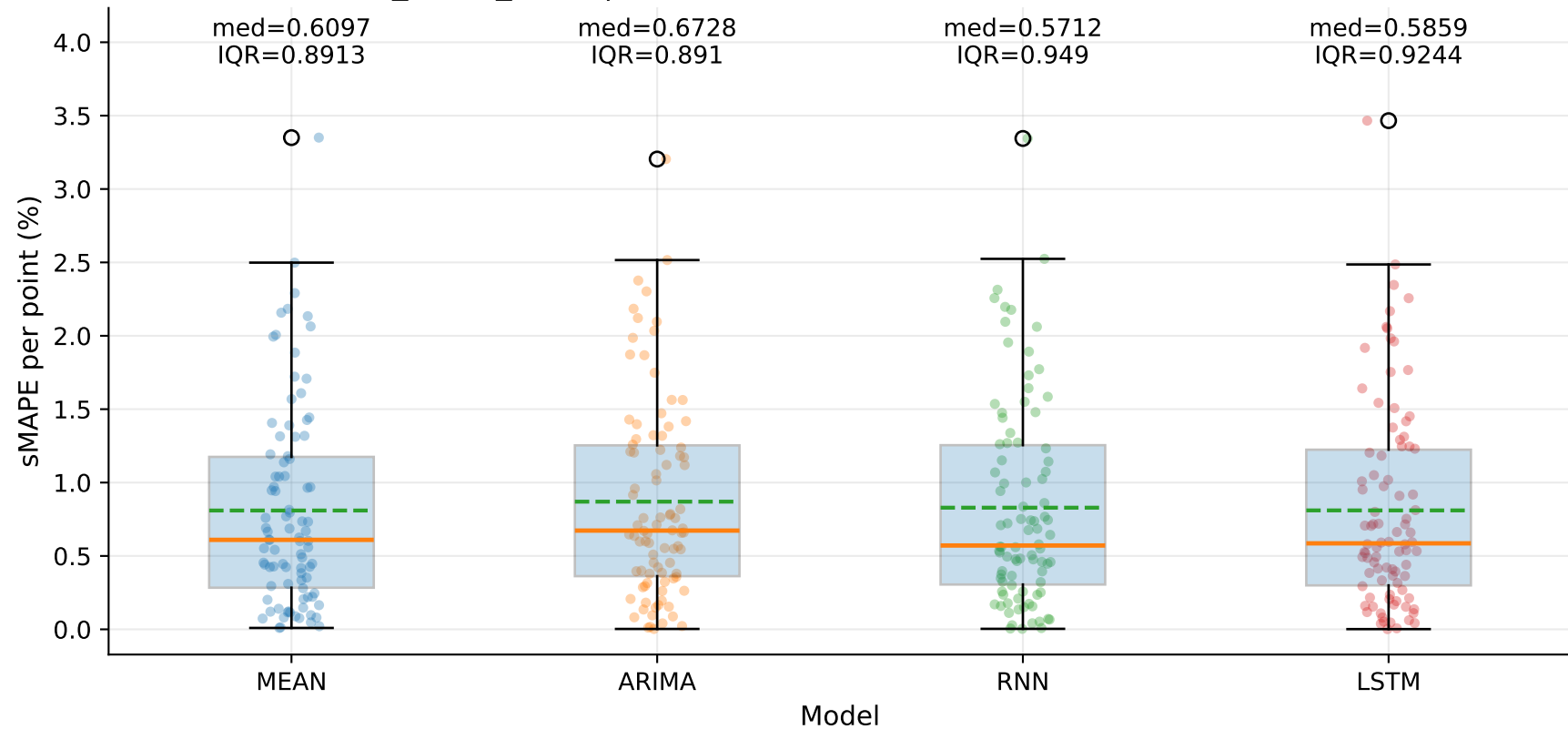
M7_YHUR_SLUR | sMAPE distribution by model — TSE (step=1)
