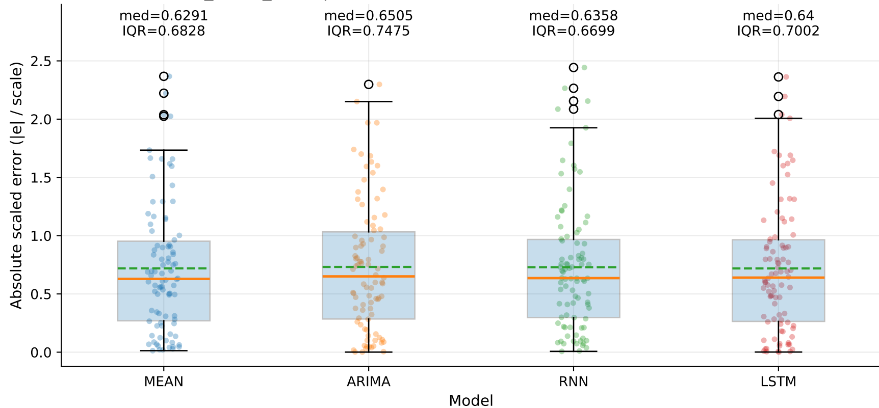
M7_YHUR_SLUR | MASE-point distribution by model — Yd (step=1)
