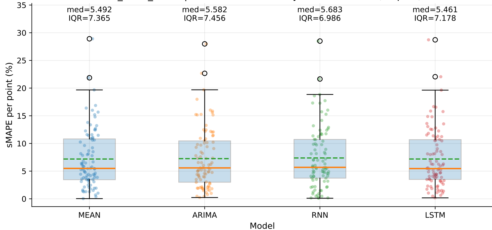
M7_YLUR_SHUR | sMAPE distribution by model — TSEC (step=1)
