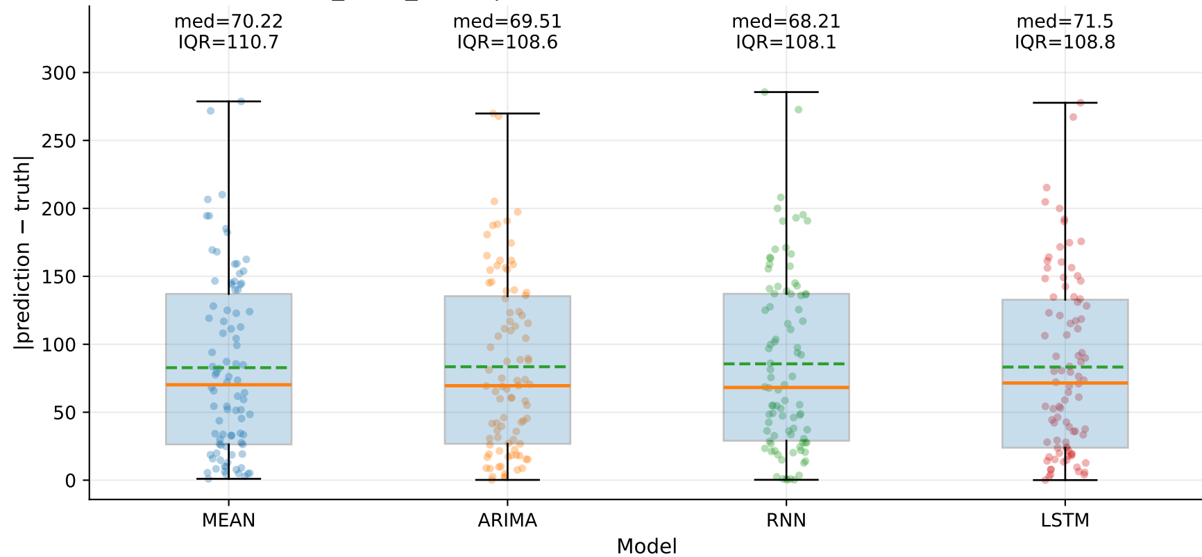
M7_YLUR_SHUR | Absolute error by model — TSE (step=1)
