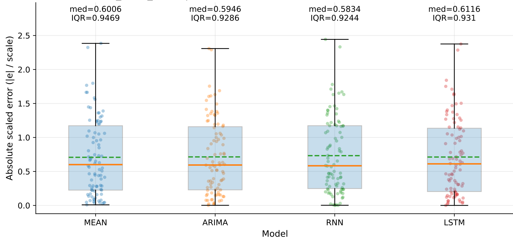
M7_YLUR_SHUR | MASE-point distribution by model — TSE (step=1)
