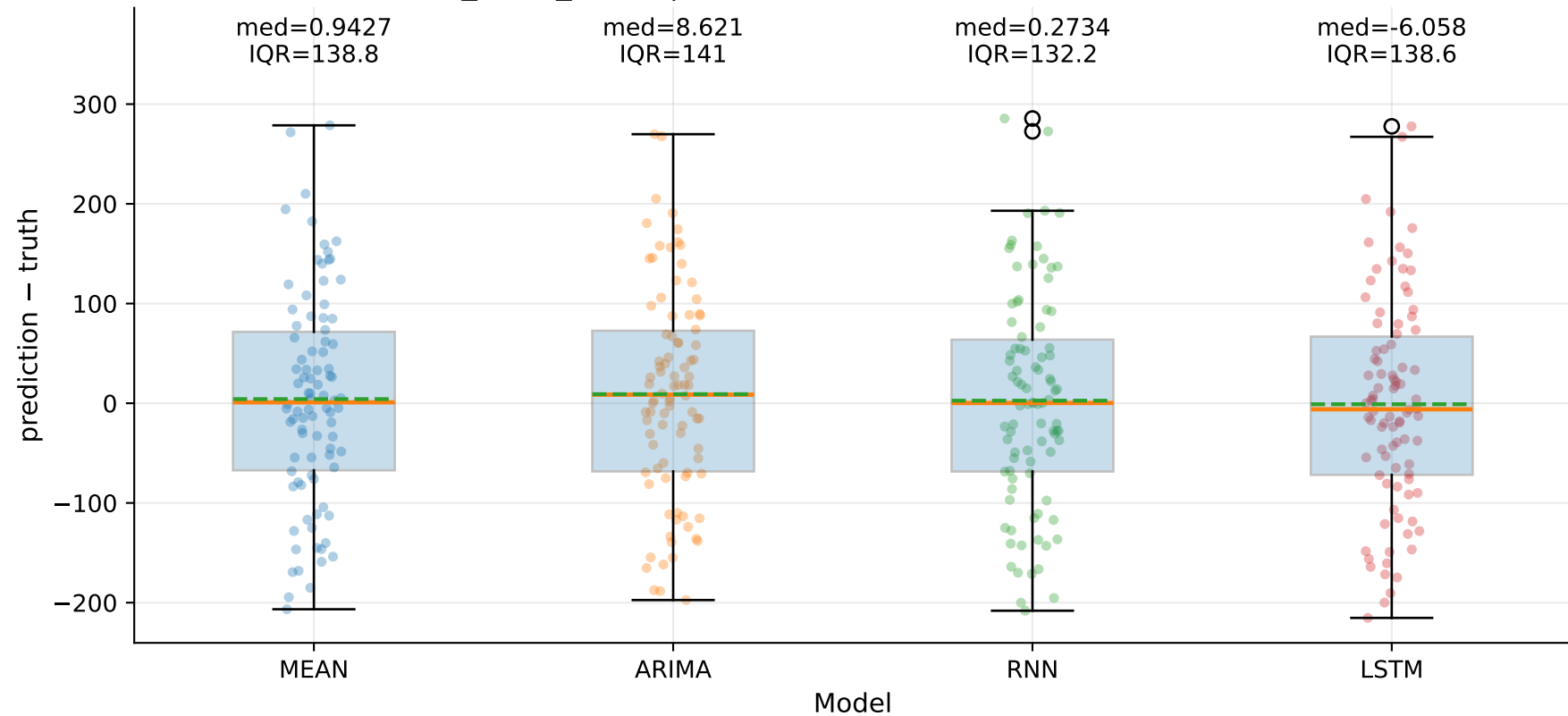
M7_YLUR_SHUR | Signed error by model — TSE (step=1)
