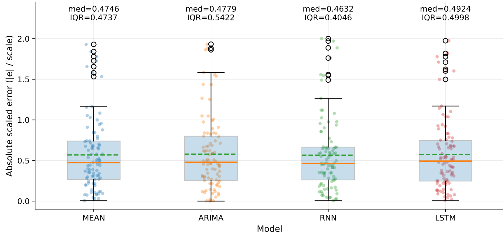
M7_YLUR_SHUR | MASE-point distribution by model — Yd (step=1)
