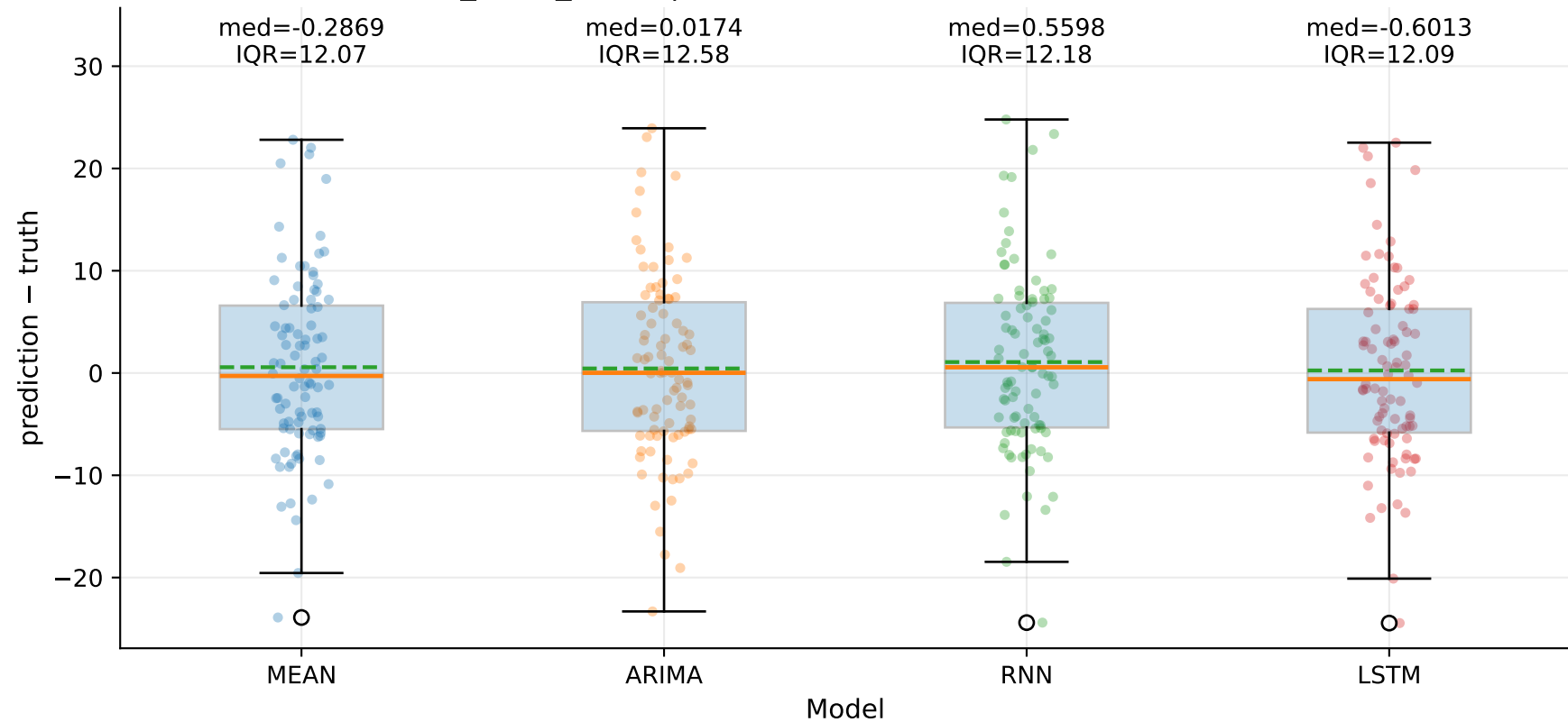
M7_YLUR_SHUR | Signed error by model — Yd (step=1)
