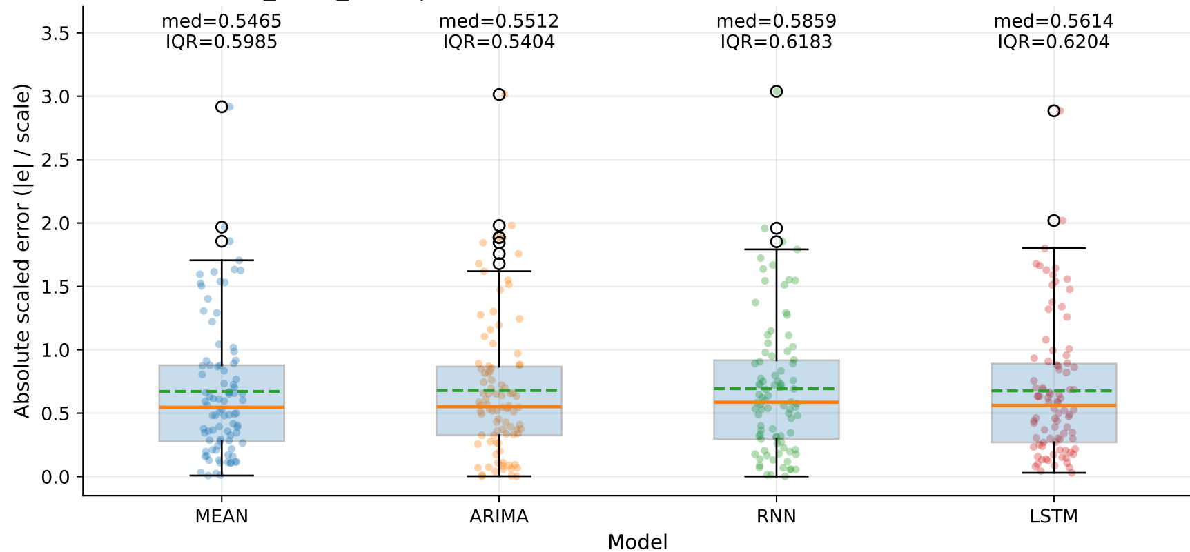
M7_YLUR_SLUR | MASE-point distribution by model — TSEC (step=1)
