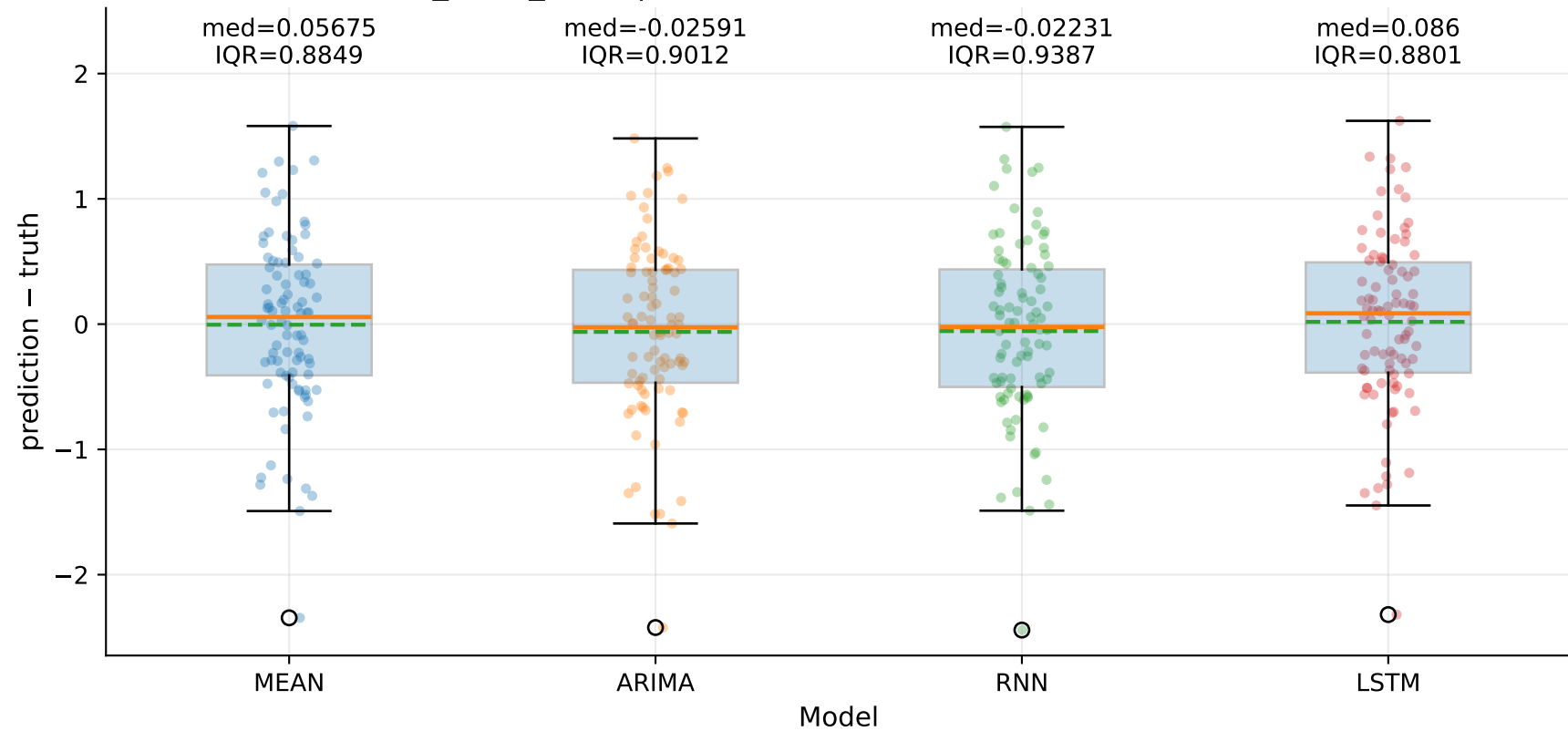
M7_YLUR_SLUR | Signed error by model — TSEC (step=1)
