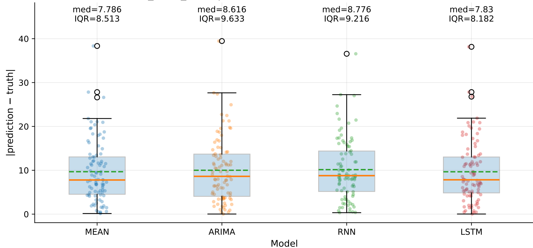
M7_YLUR_SLUR | Absolute error by model — Yd (step=1)
