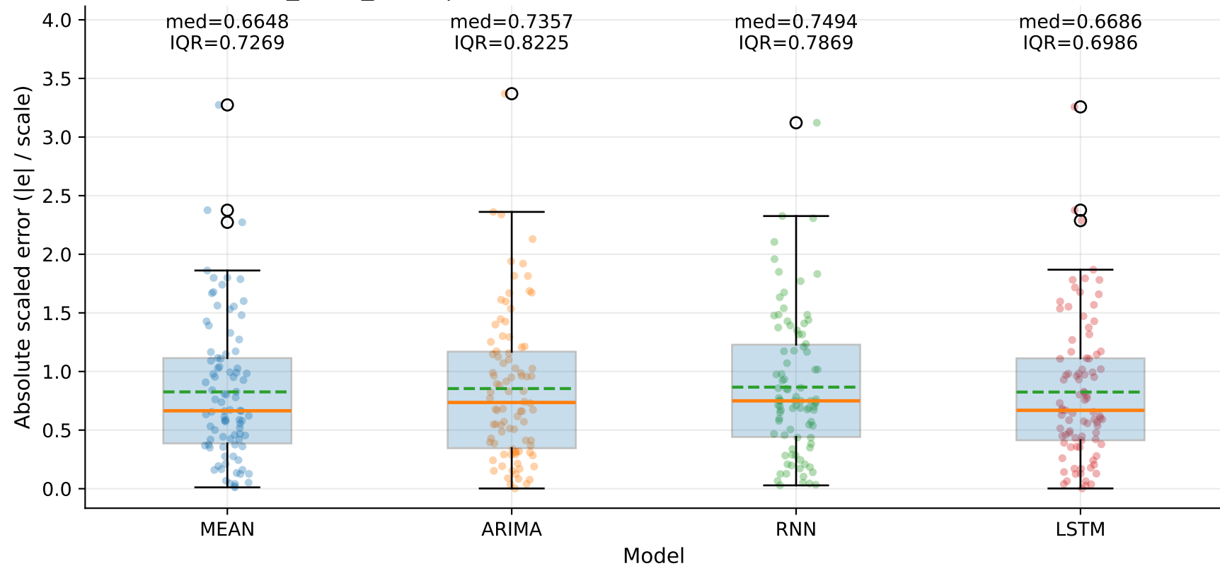
M7_YLUR_SLUR | MASE-point distribution by model — Yd (step=1)
