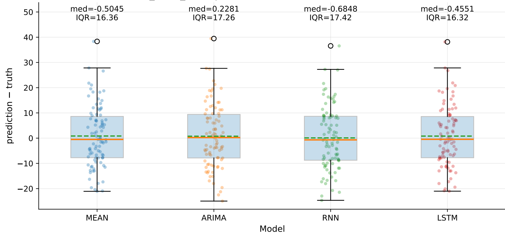
M7_YLUR_SLUR | Signed error by model — Yd (step=1)
