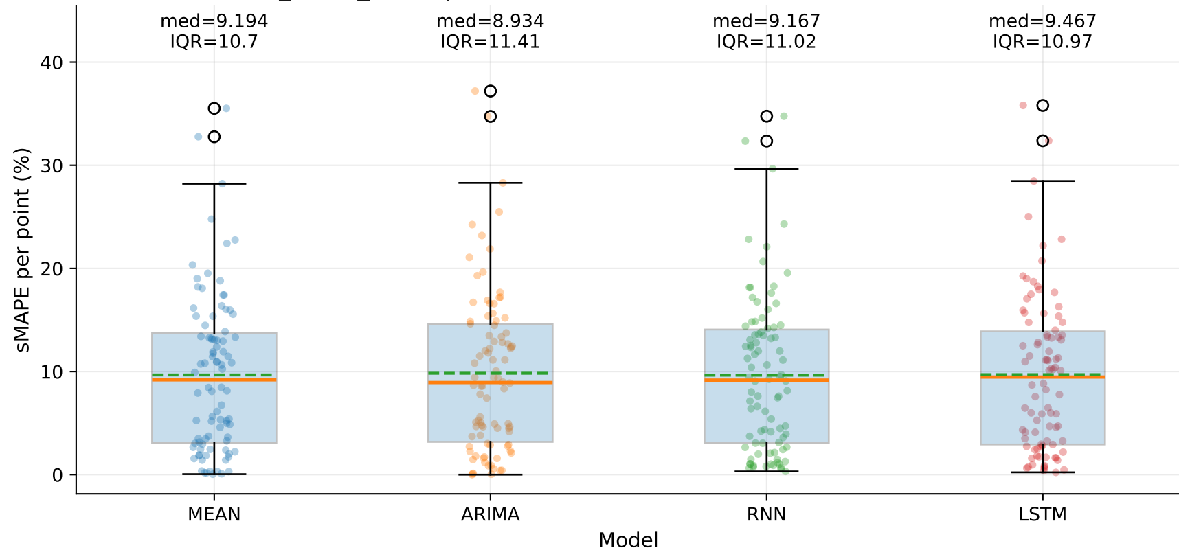
M8_YHUR_SHUR | sMAPE distribution by model — TSEC (step=1)
