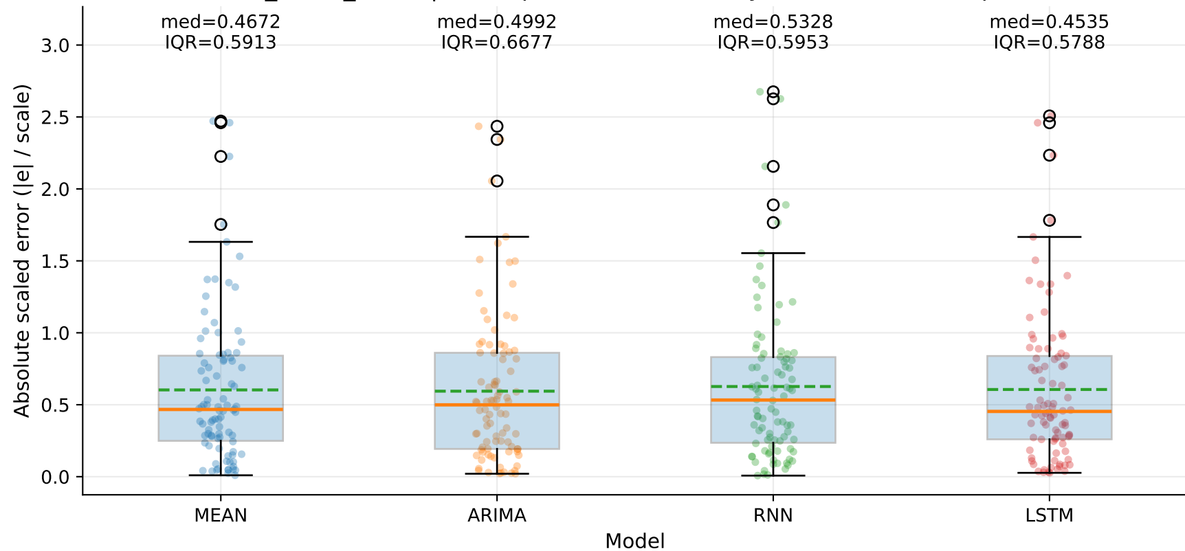
M8_YHUR_SHUR | MASE-point distribution by model — TSE (step=1)
