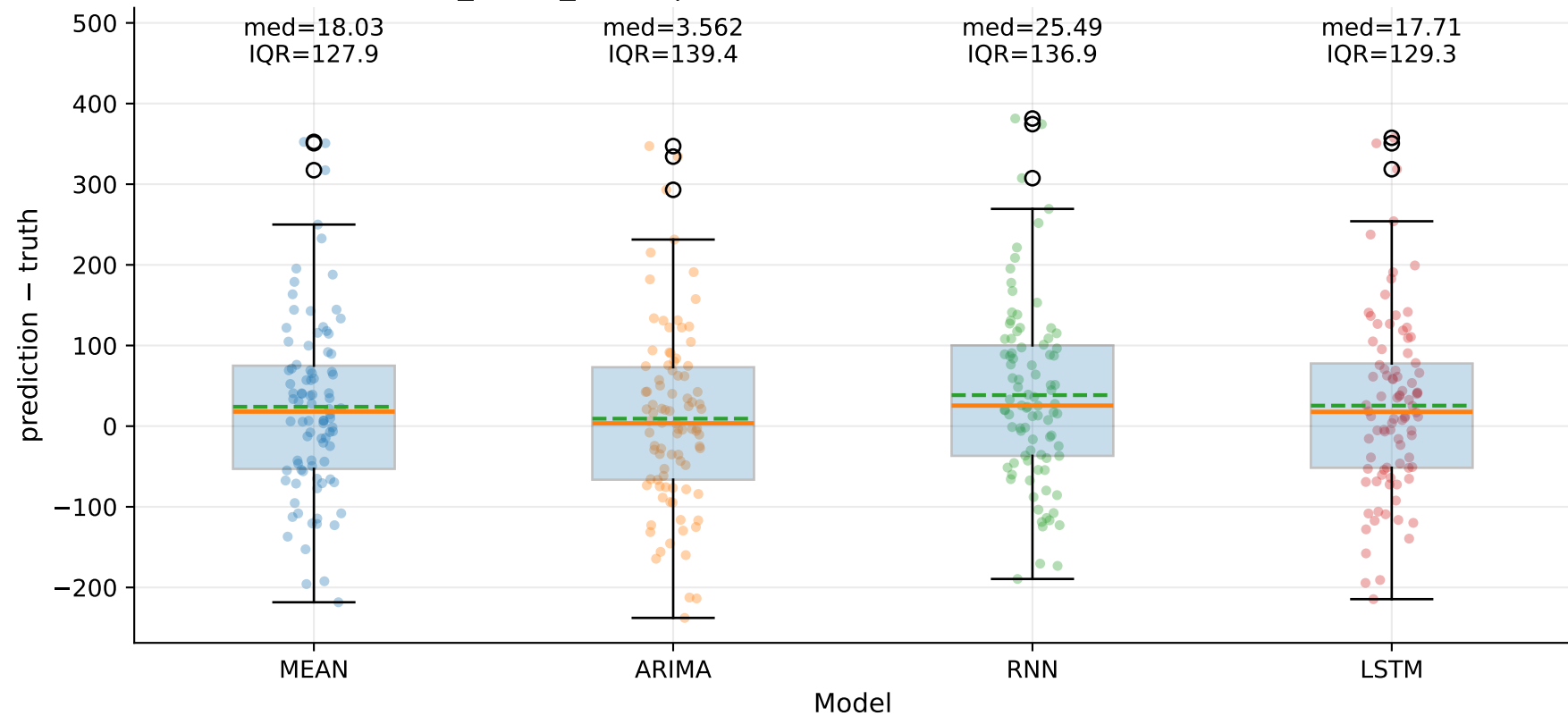
M8_YHUR_SHUR | Signed error by model — TSE (step=1)
