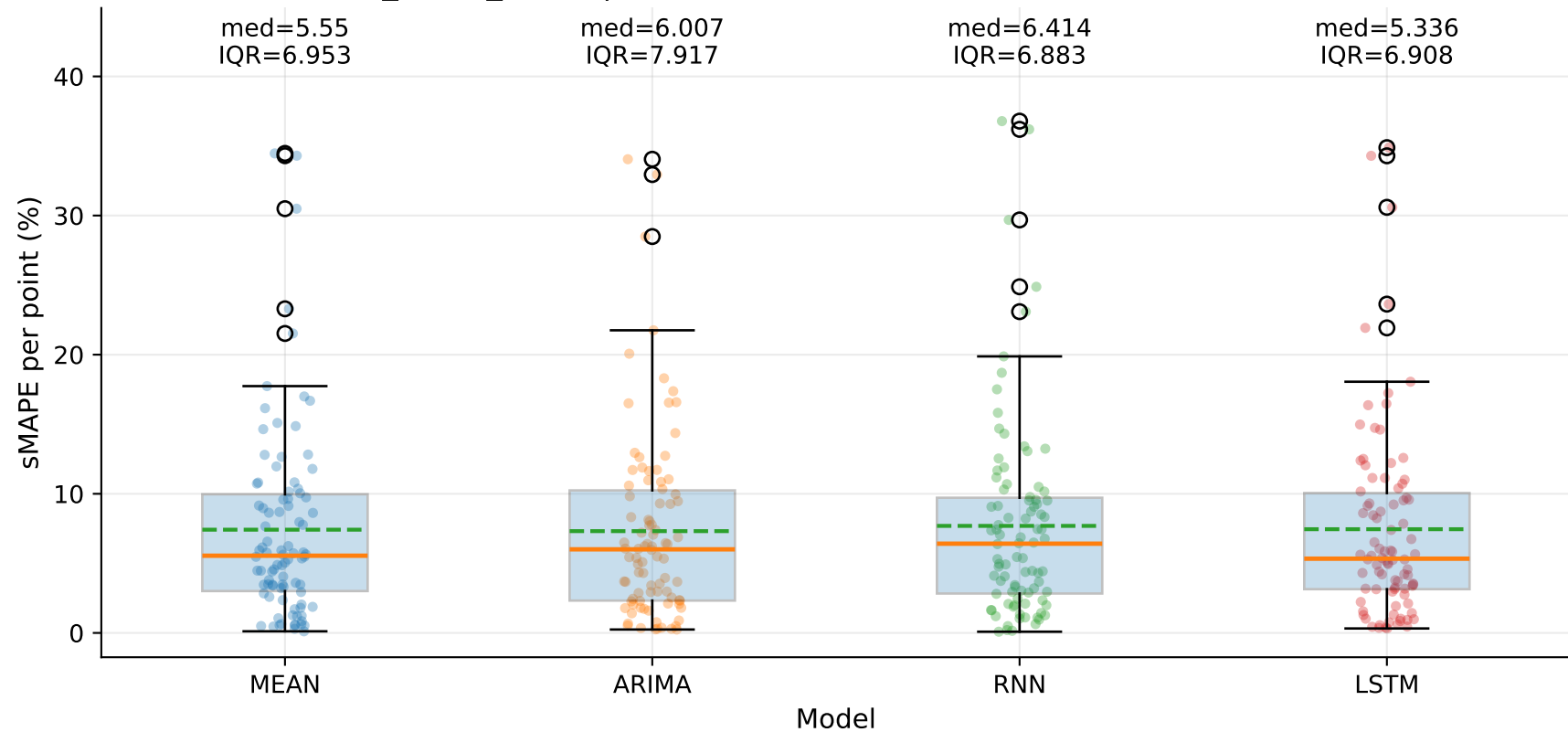
M8_YHUR_SHUR | sMAPE distribution by model — TSE (step=1)
