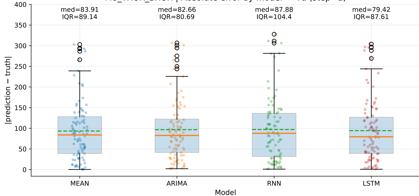
M8_YHUR_SHUR | Absolute error by model — Yd (step=1)
