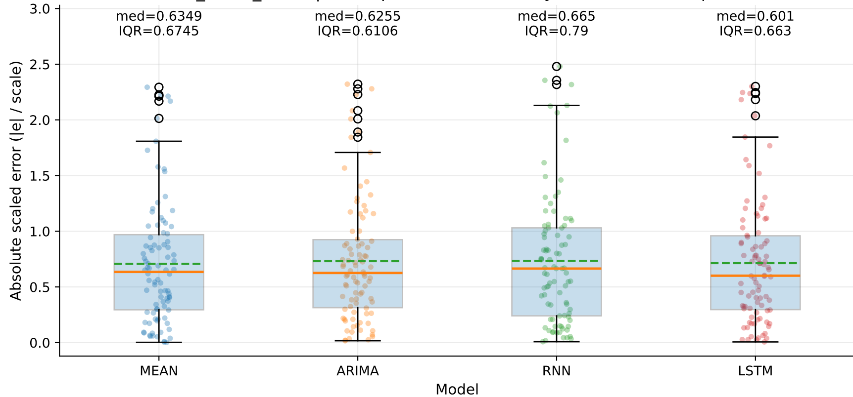
M8_YHUR_SHUR | MASE-point distribution by model — Yd (step=1)
