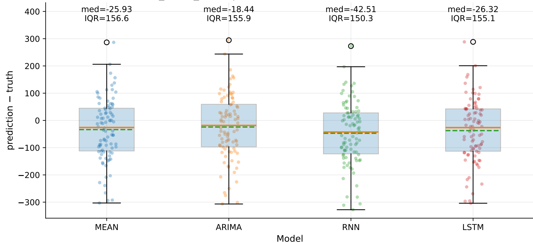
M8_YHUR_SHUR | Signed error by model — Yd (step=1)
