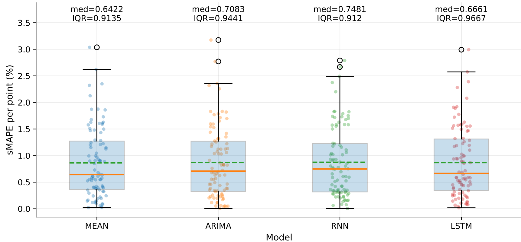
M8_YHUR_SLUR | sMAPE distribution by model — TSEC (step=1)
