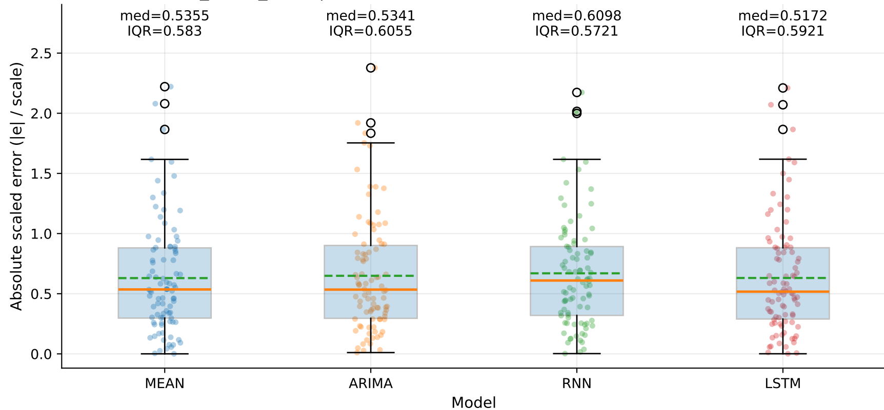
M8_YHUR_SLUR | MASE-point distribution by model — TSE (step=1)
