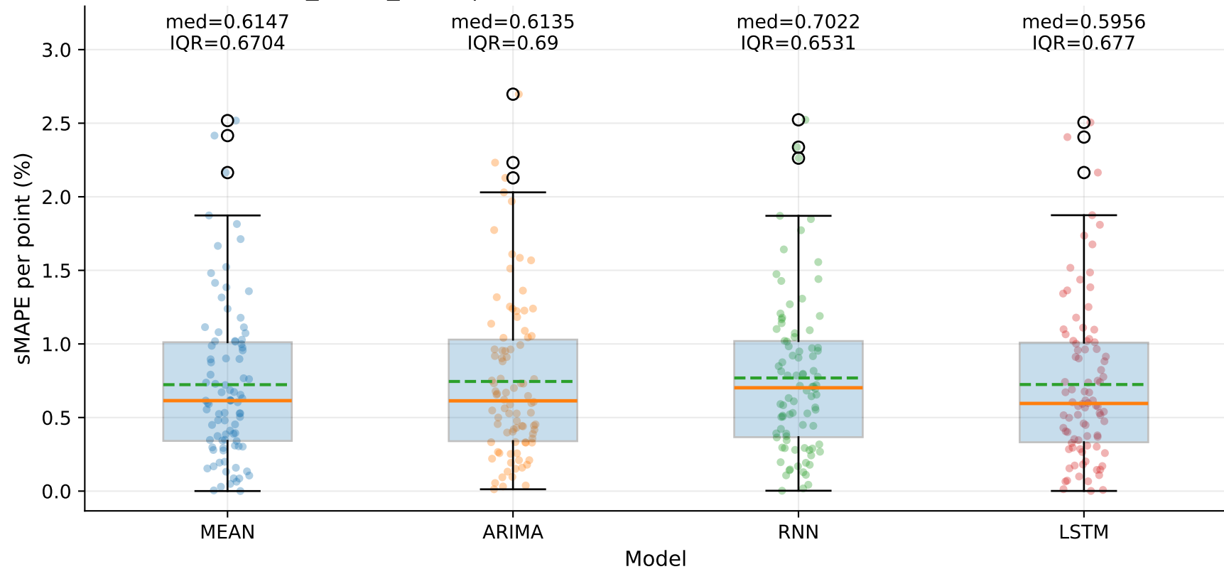
M8_YHUR_SLUR | sMAPE distribution by model — TSE (step=1)
