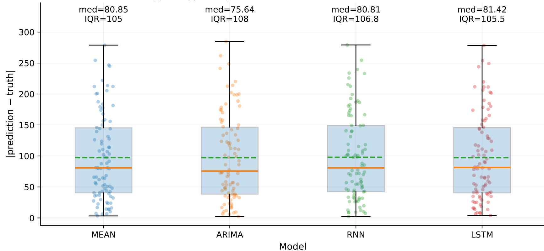
M8_YHUR_SLUR | Absolute error by model — Yd (step=1)
