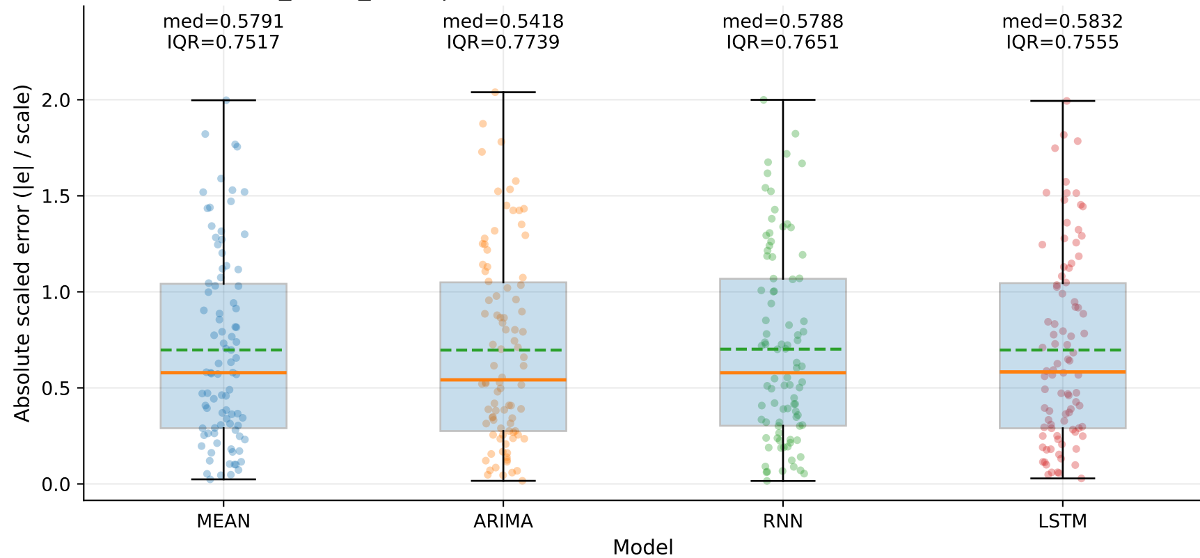
M8_YHUR_SLUR | MASE-point distribution by model — Yd (step=1)
