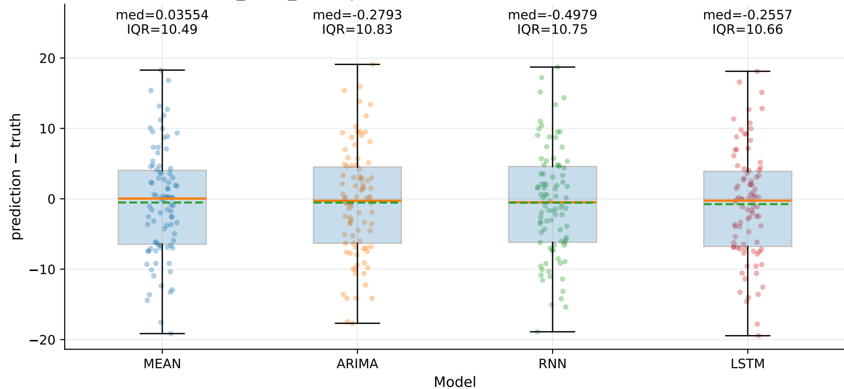
M8_YLUR_SHUR | Signed error by model — TSEC (step=1)
