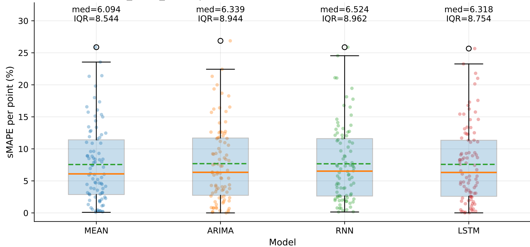
M8_YLUR_SHUR | sMAPE distribution by model — TSEC (step=1)
