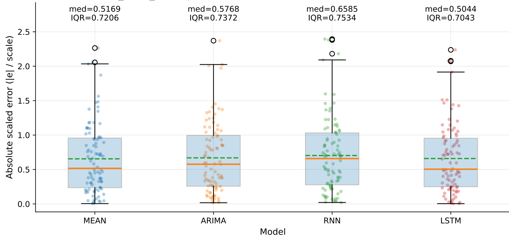
M8_YLUR_SHUR | MASE-point distribution by model — Yd (step=1)
