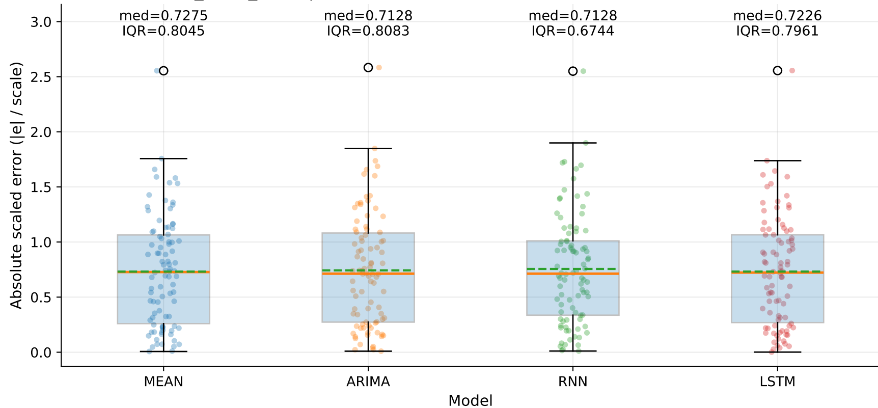
M8_YLUR_SLUR | MASE-point distribution by model — TSEC (step=1)
