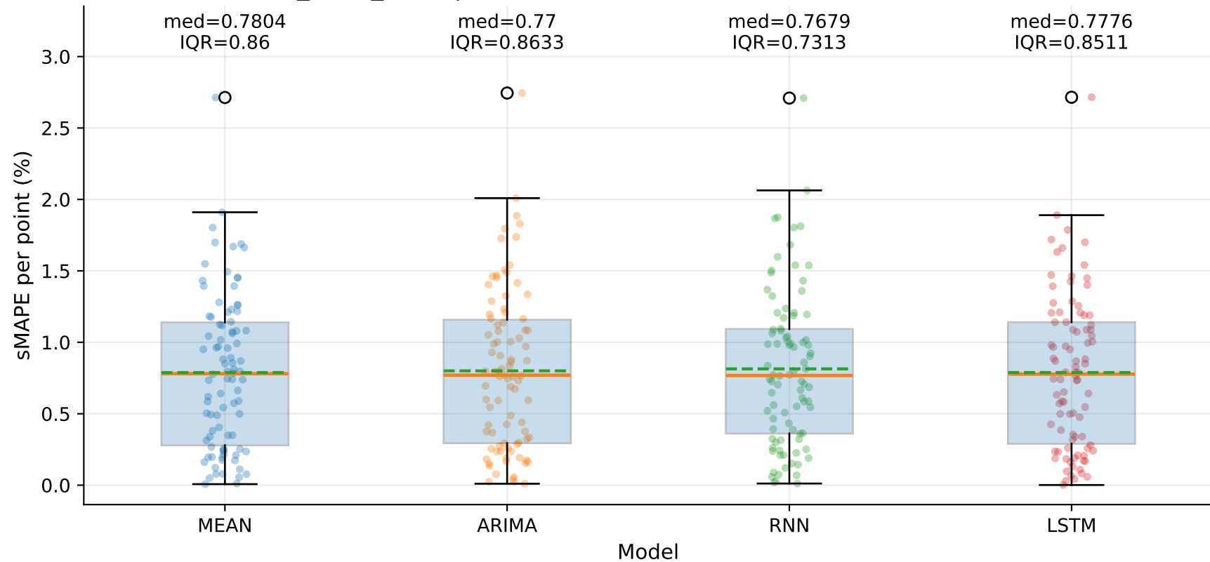
M8_YLUR_SLUR | sMAPE distribution by model — TSEC (step=1)
