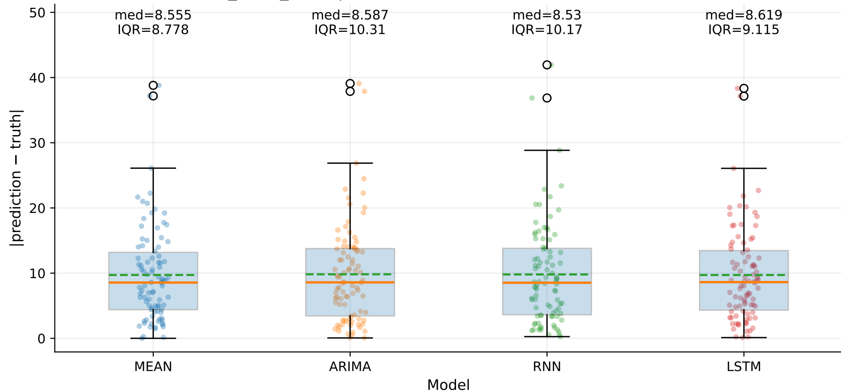
M8_YLUR_SLUR | Absolute error by model — TSE (step=1)
