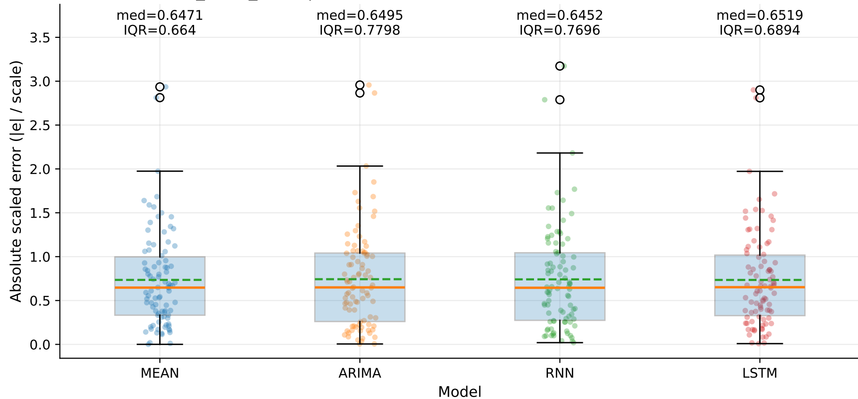
M8_YLUR_SLUR | MASE-point distribution by model — TSE (step=1)
