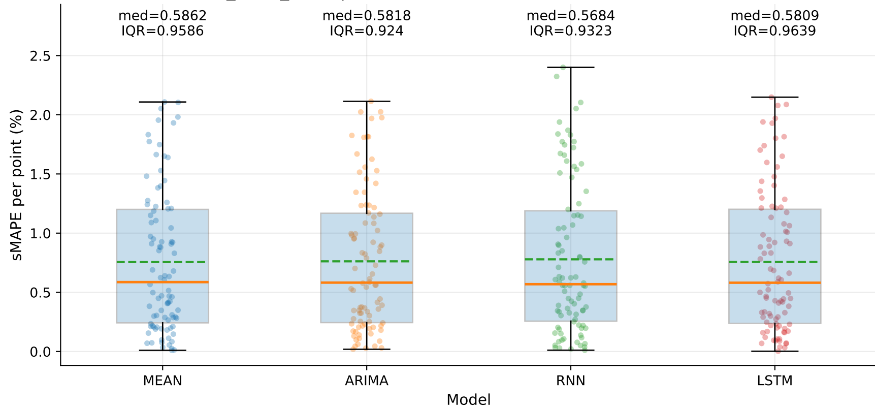
M8_YLUR_SLUR | sMAPE distribution by model — Yd (step=1)
