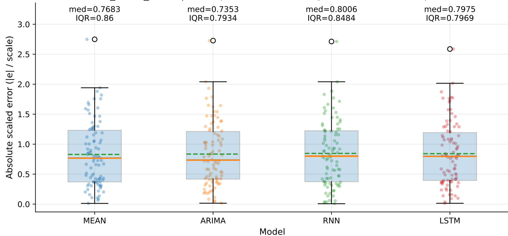
M9_YHUR_SHUR | MASE-point distribution by model — TSEC (step=1)
