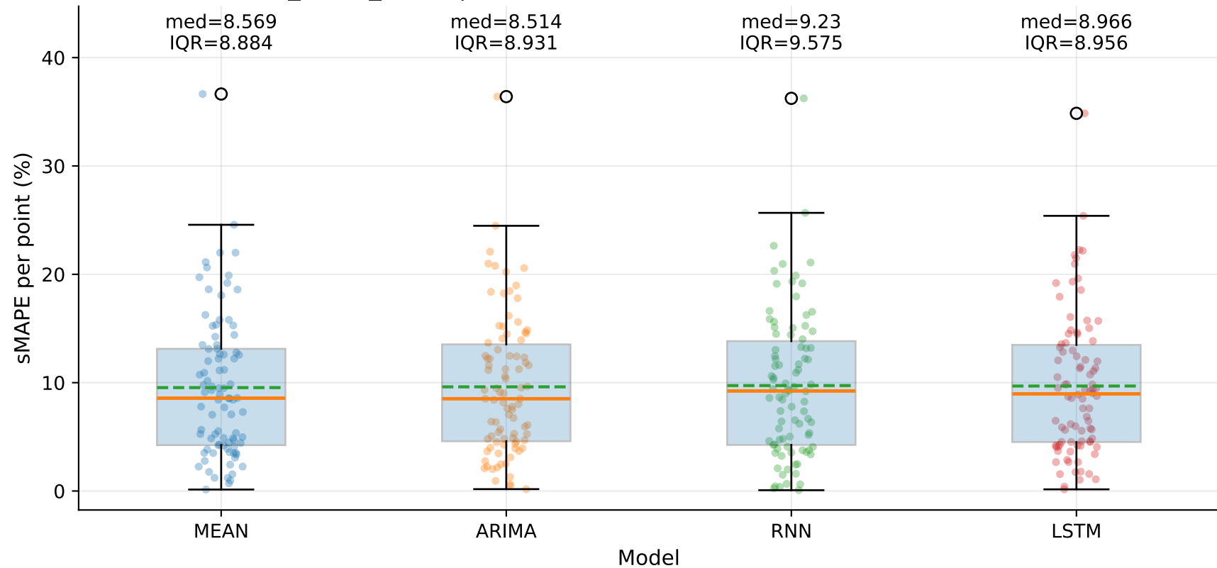
M9_YHUR_SHUR | sMAPE distribution by model — TSEC (step=1)
