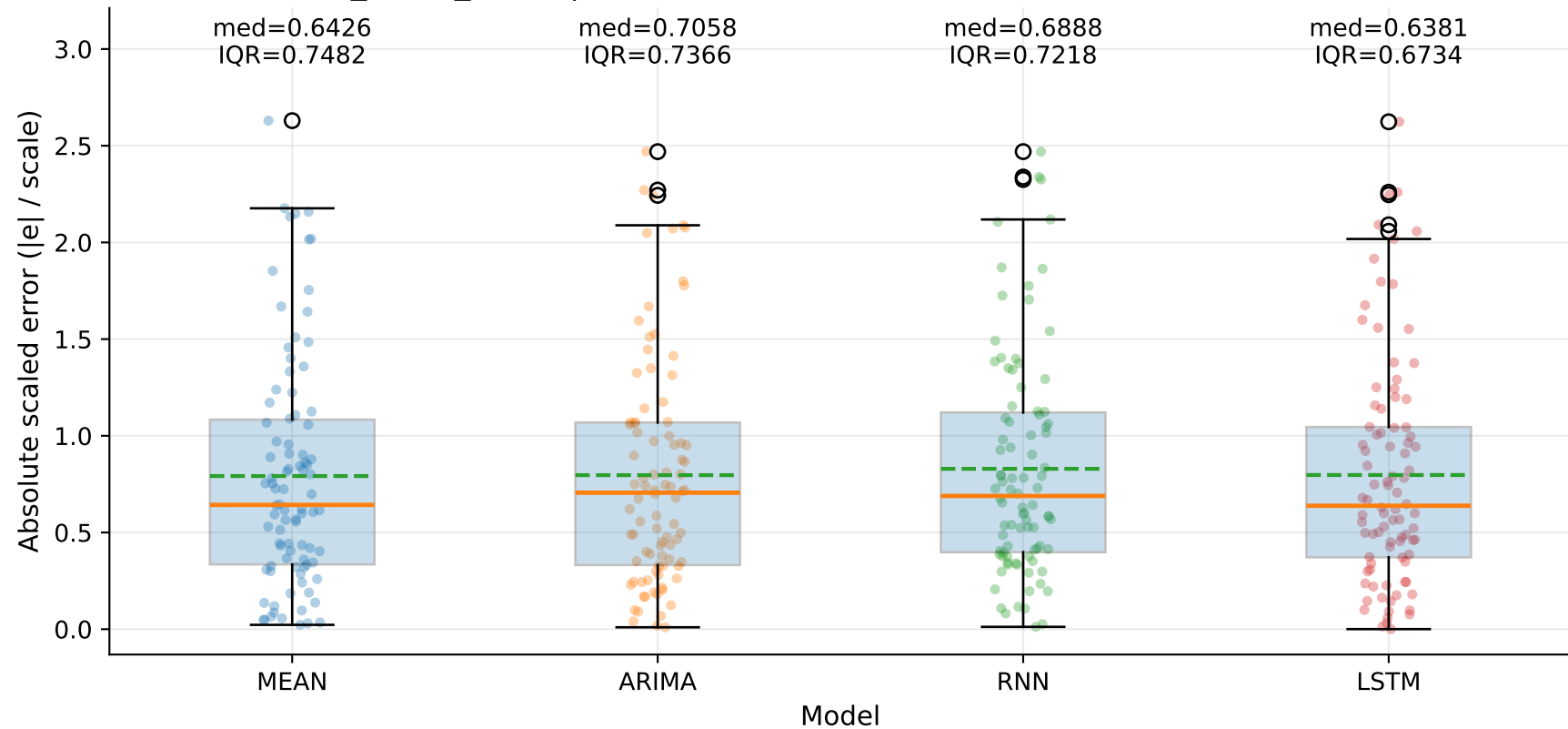
M9_YHUR_SHUR | MASE-point distribution by model — TSE (step=1)
