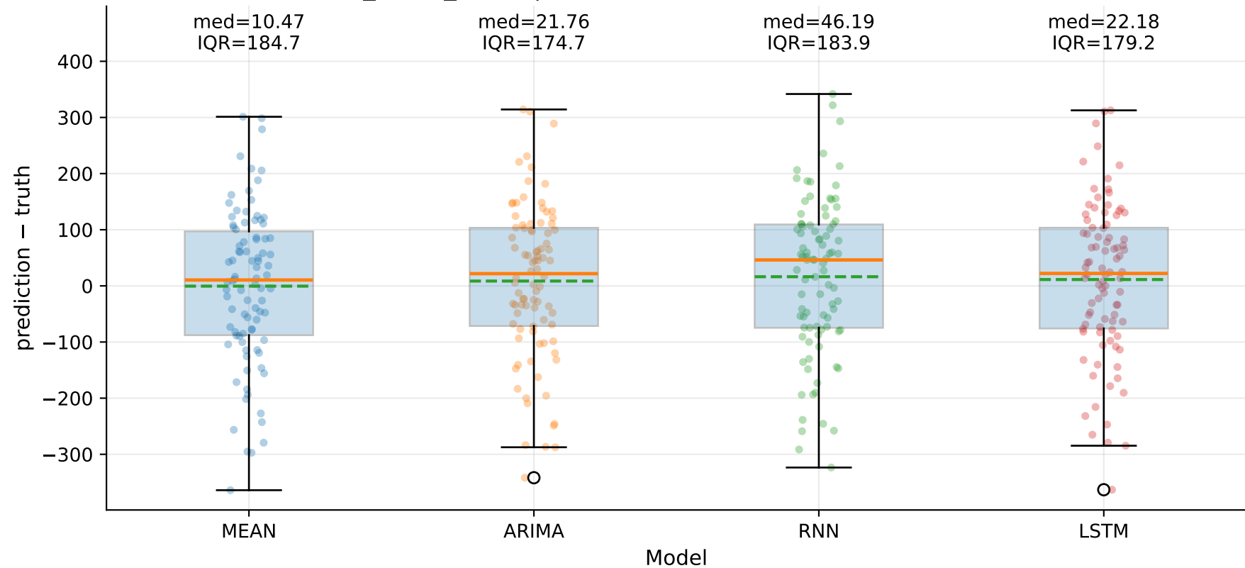
M9_YHUR_SHUR | Signed error by model — TSE (step=1)
