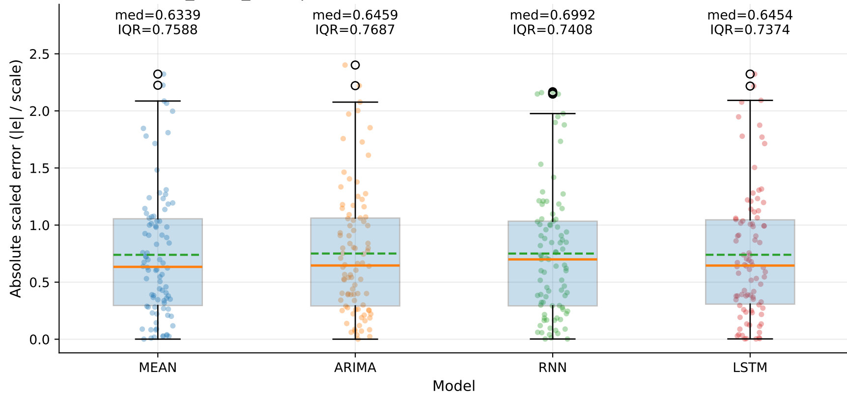
M9_YHUR_SLUR | MASE-point distribution by model — TSEC (step=1)
