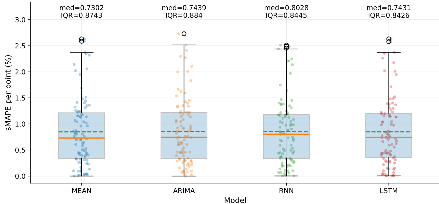
M9_YHUR_SLUR | sMAPE distribution by model — TSEC (step=1)
