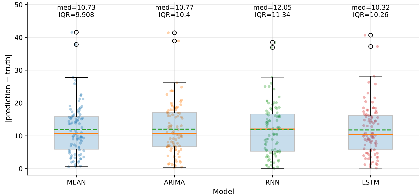
M9_YHUR_SLUR | Absolute error by model — TSE (step=1)
