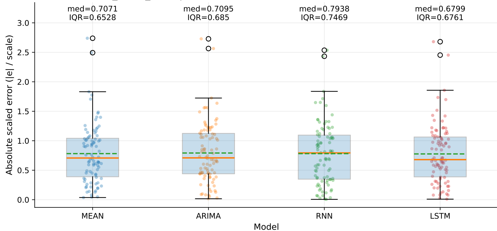
M9_YHUR_SLUR | MASE-point distribution by model — TSE (step=1)
