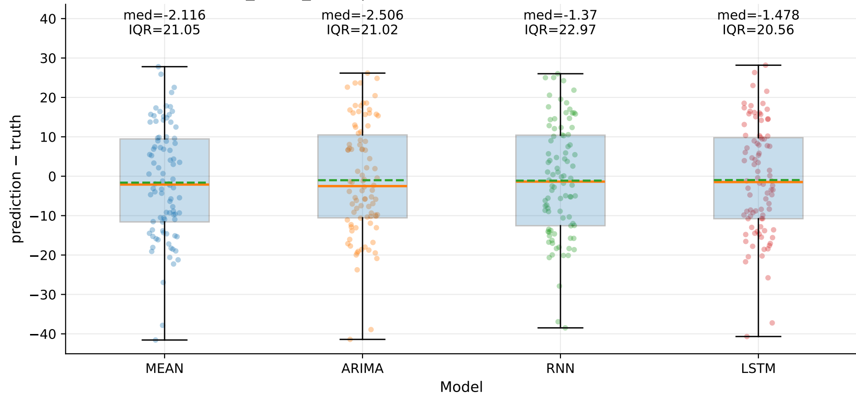
M9_YHUR_SLUR | Signed error by model — TSE (step=1)
