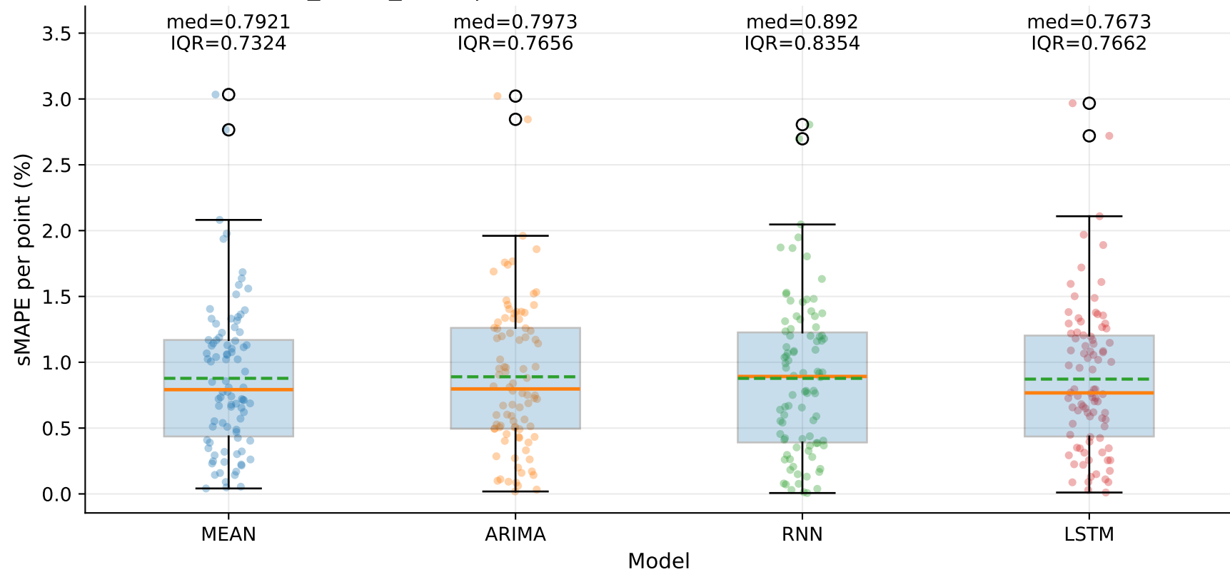
M9_YHUR_SLUR | sMAPE distribution by model — TSE (step=1)
