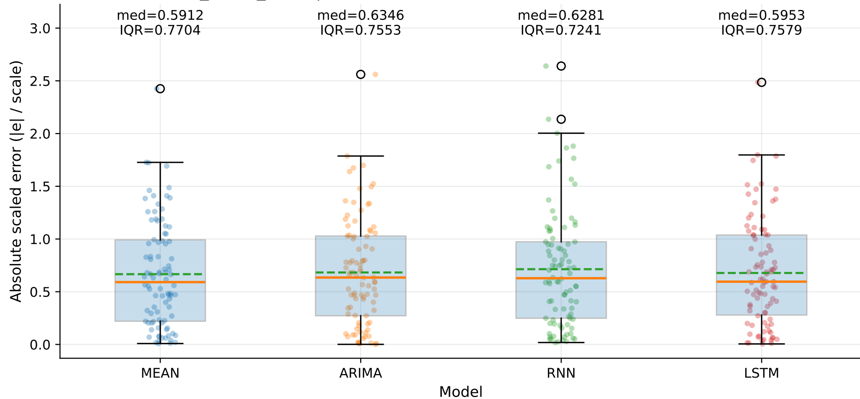
M9_YHUR_SLUR | MASE-point distribution by model — Yd (step=1)
