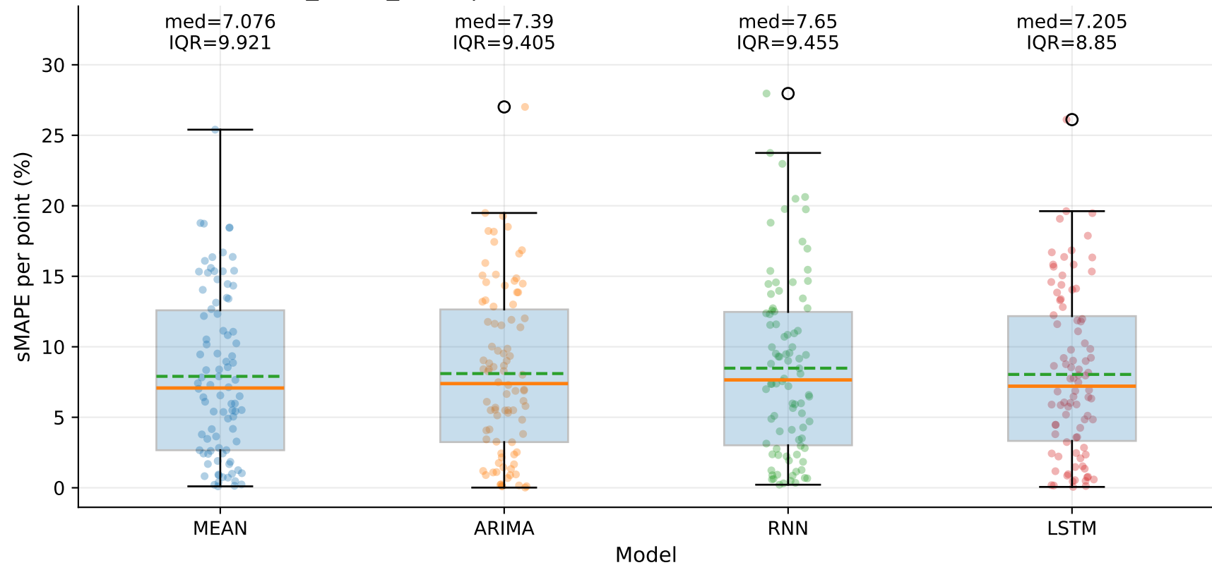
M9_YHUR_SLUR | sMAPE distribution by model — Yd (step=1)
