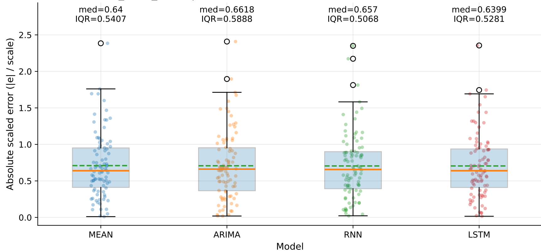
M9_YLUR_SHUR | MASE-point distribution by model — TSEC (step=1)
