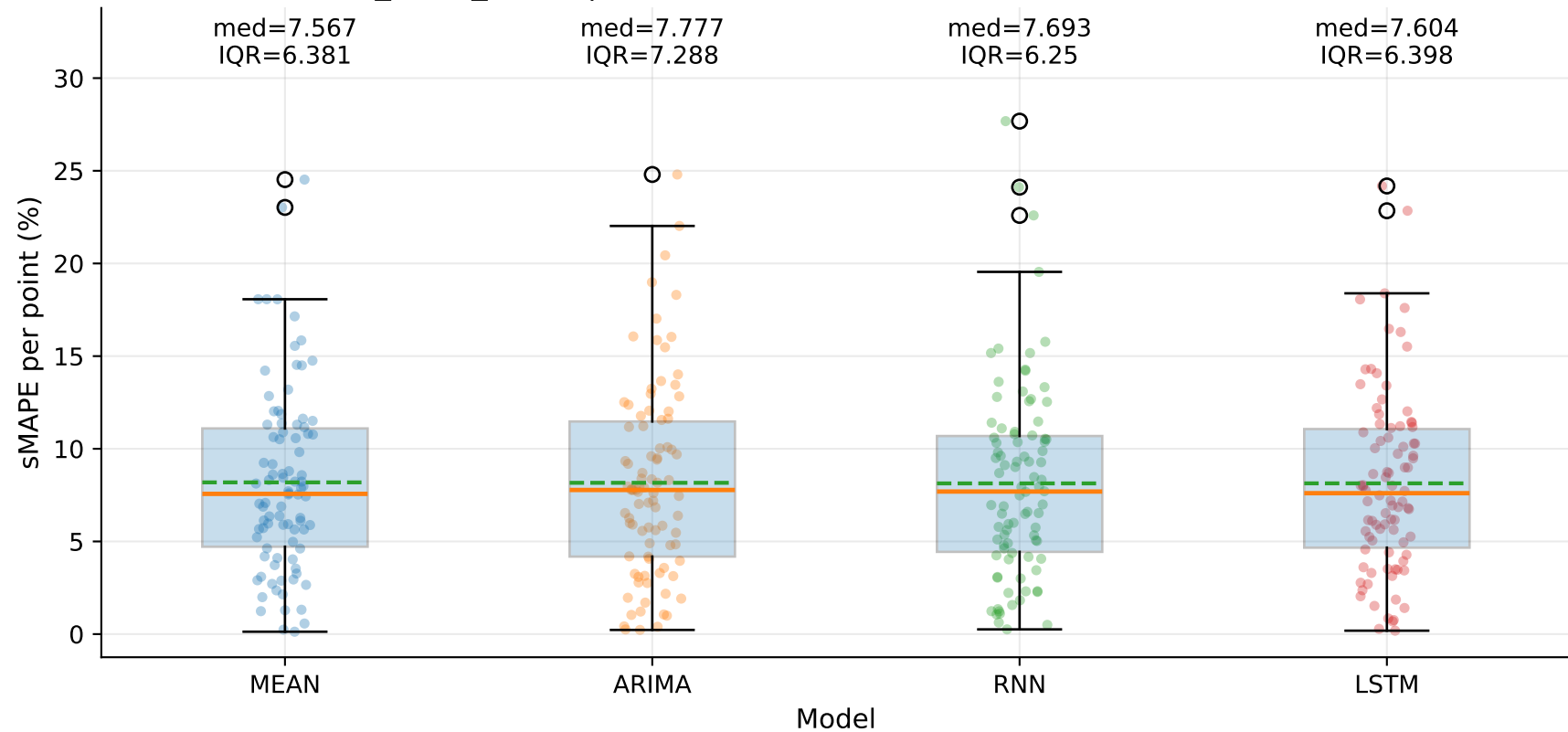
M9_YLUR_SHUR | sMAPE distribution by model — TSEC (step=1)
