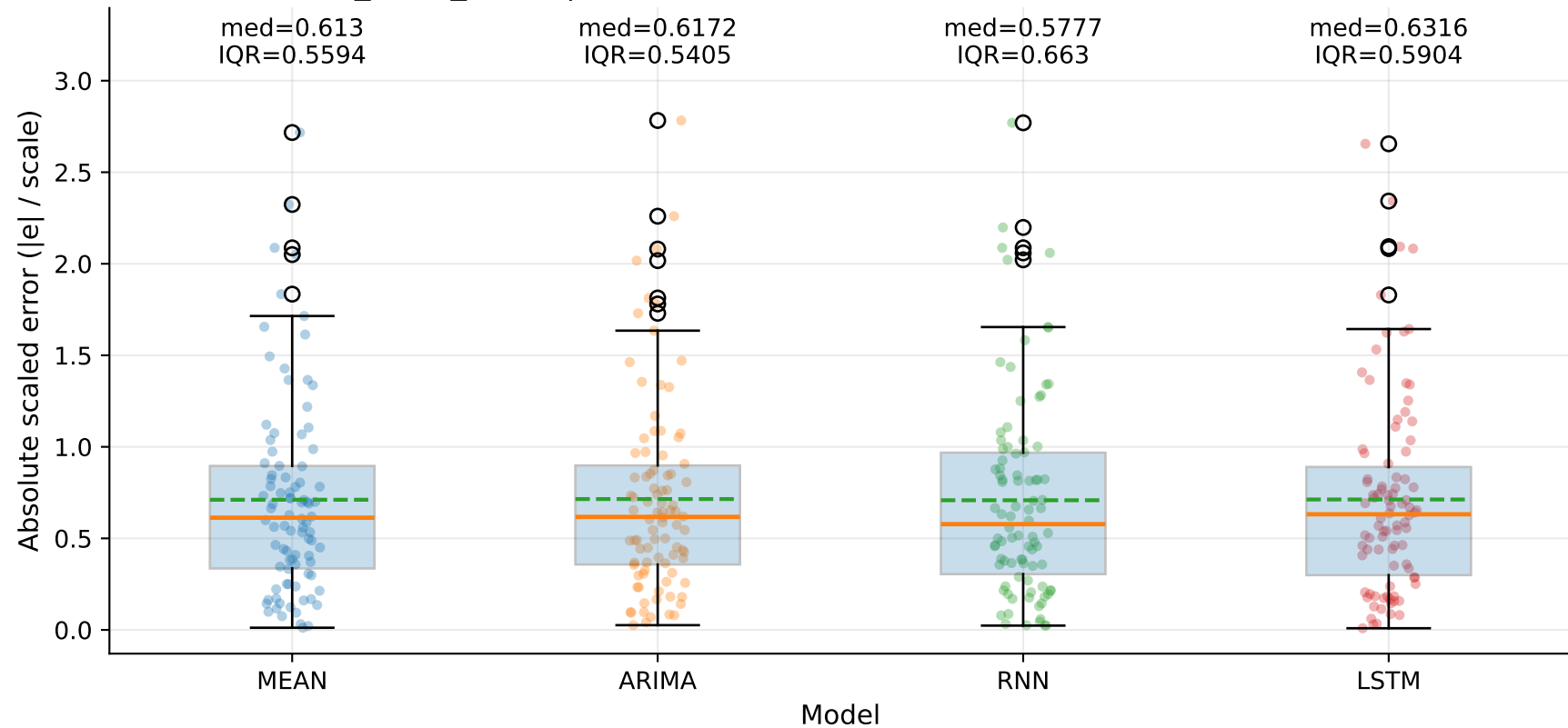
M9_YLUR_SHUR | MASE-point distribution by model — TSE (step=1)
