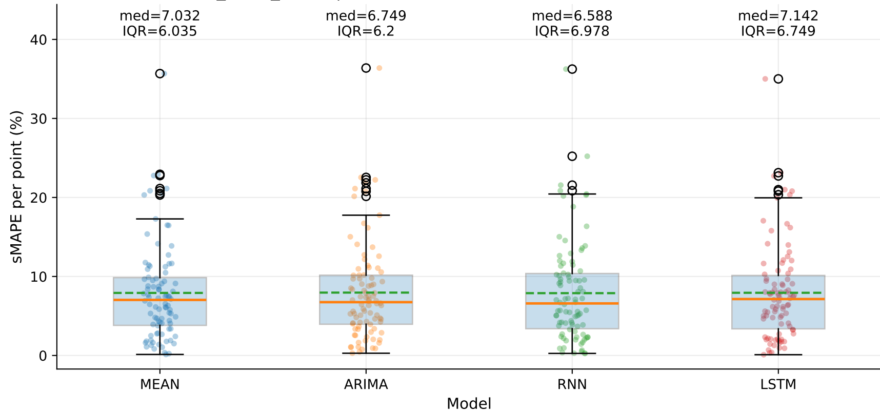
M9_YLUR_SHUR | sMAPE distribution by model — TSE (step=1)
